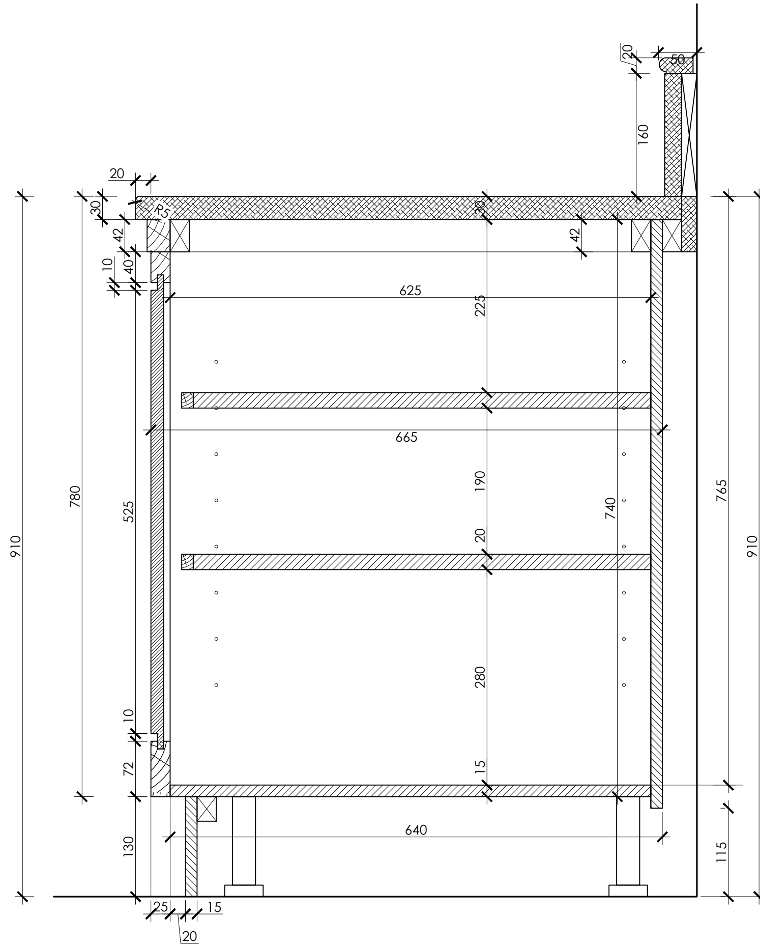
Cupboard Unit Section 1:5
