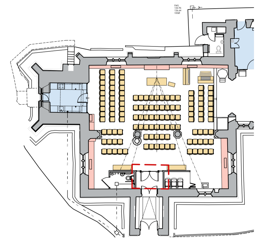
Ground Floor Plan 1:200 1:200 metres 4 8 12 16 20
